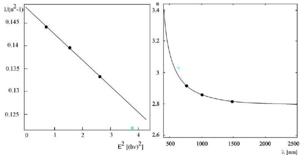
Figure 4. 1/(n^2-1) dependence on (h\nu)^2 and the dispersion of the refractive index based on the Wemple and DiDomenico model of the amorphous \text{Cu}_{20}((\text{As}_2\text{Se}_3)_{0.9}(\text{AsI})_{0.1})_{80} thin film
