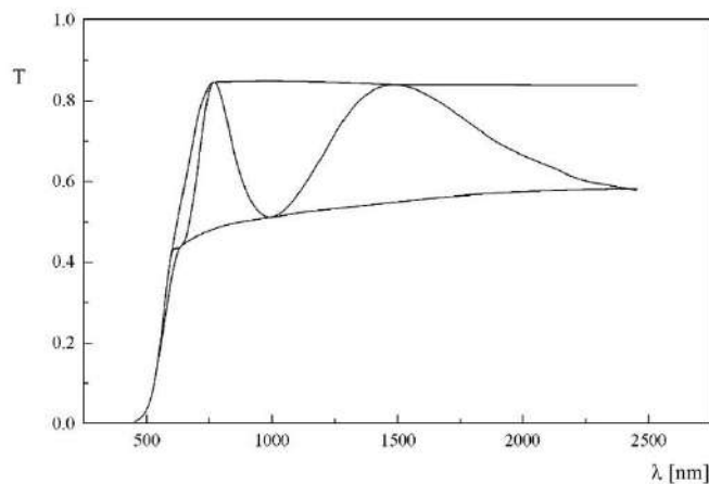
Figure 2. Transmission spectrum of the \text{Cu}_{20}((\text{As}_2\text{Se}_3)_{0.9}(\text{AsI})_{0.1})_{80} amorphous thin film on glass substrate.
